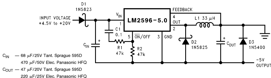
FIGURE 25. Inverting -5V Regulator with Delayed Startup
