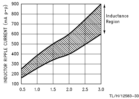
FIGURE 18. Peak-to-Peak Inductor Ripple Current vs Load Current
